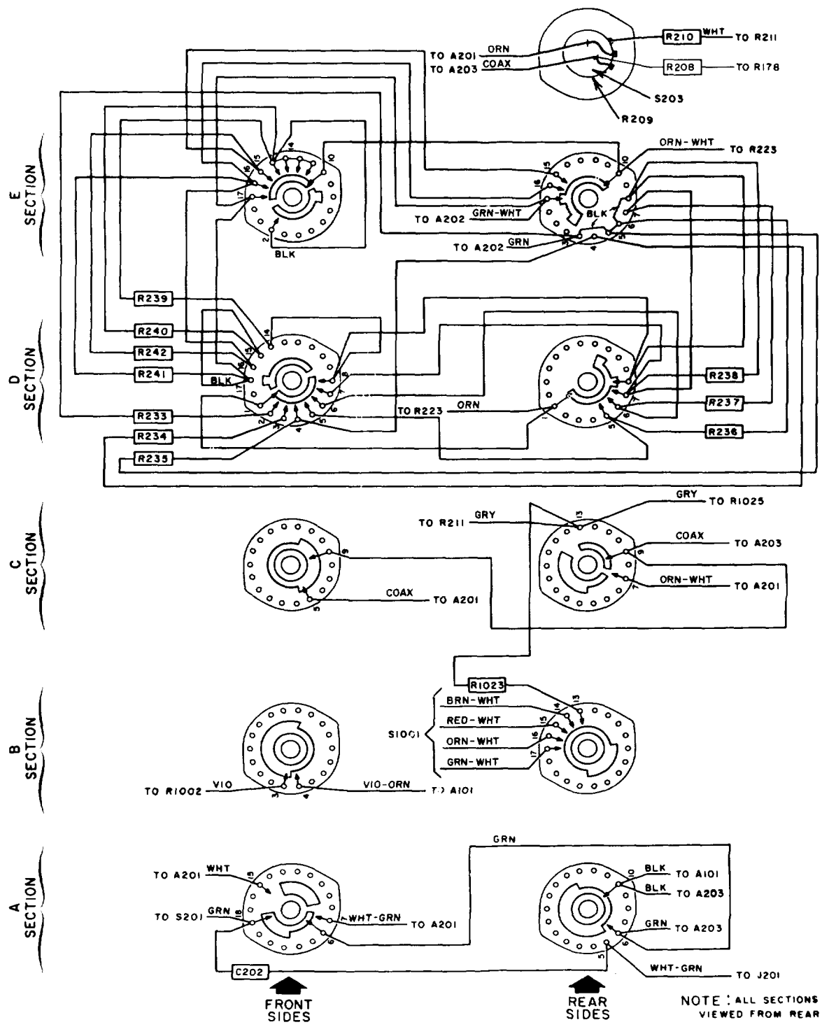
Figure 5-42A. Horizontal Display Switch Schematic Diagram AN/USM-140C
