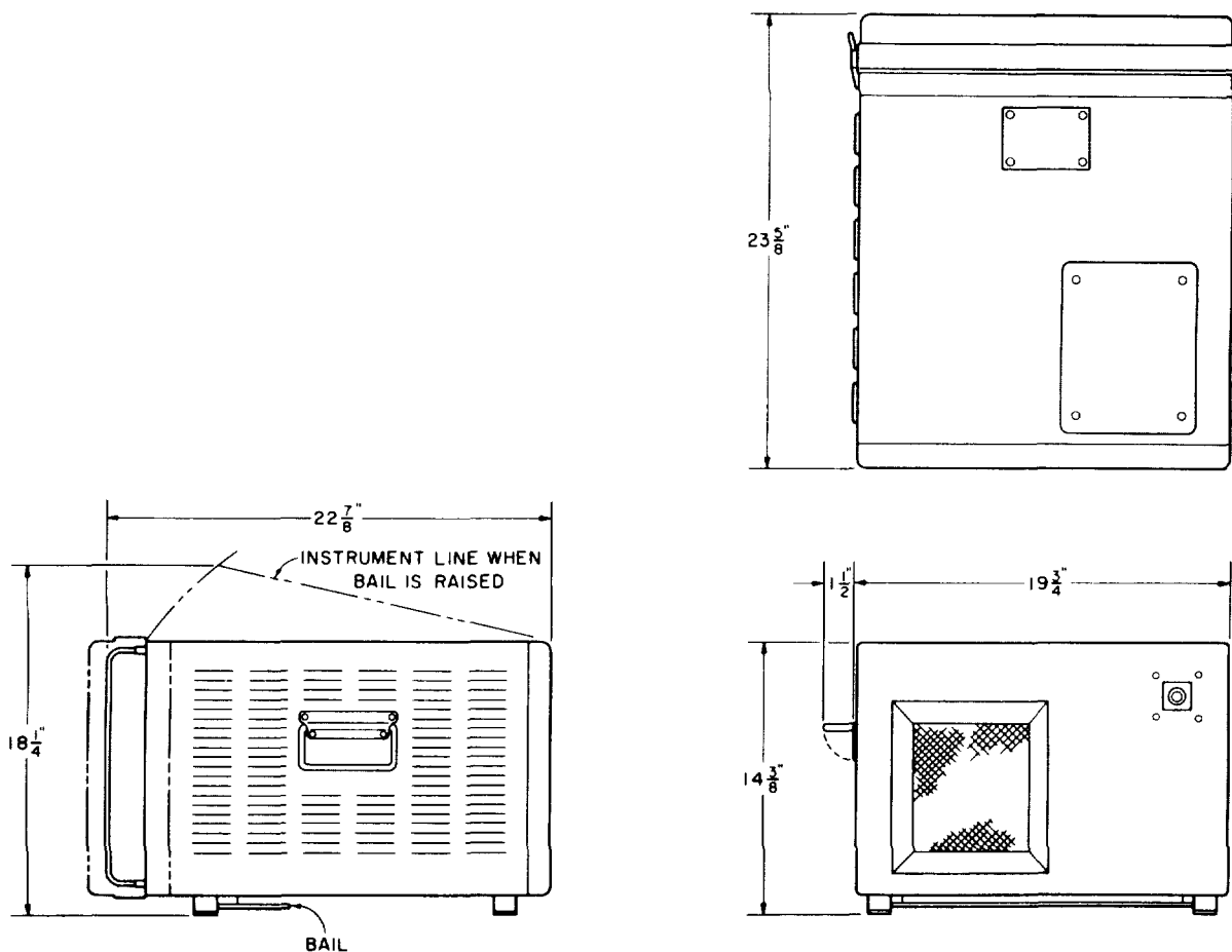
Figure 2-2. AN/USM-140B Dimensions
