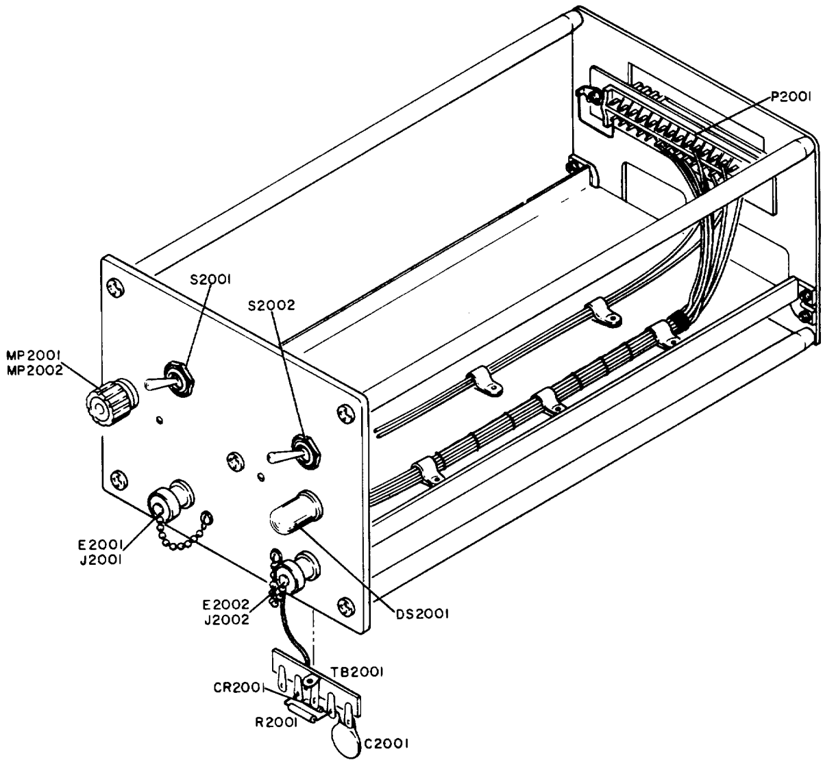
Figure 5-36. MX-3078/USM Horizontal Auxiliary Plug-In Unit, Location of Parts
